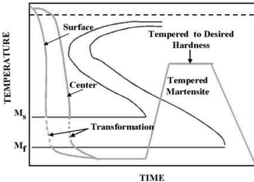
Figure 2.18 Conventional quenching and tempering process.
