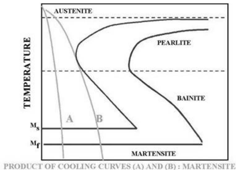
Figure 2.9. Rapid Quench
