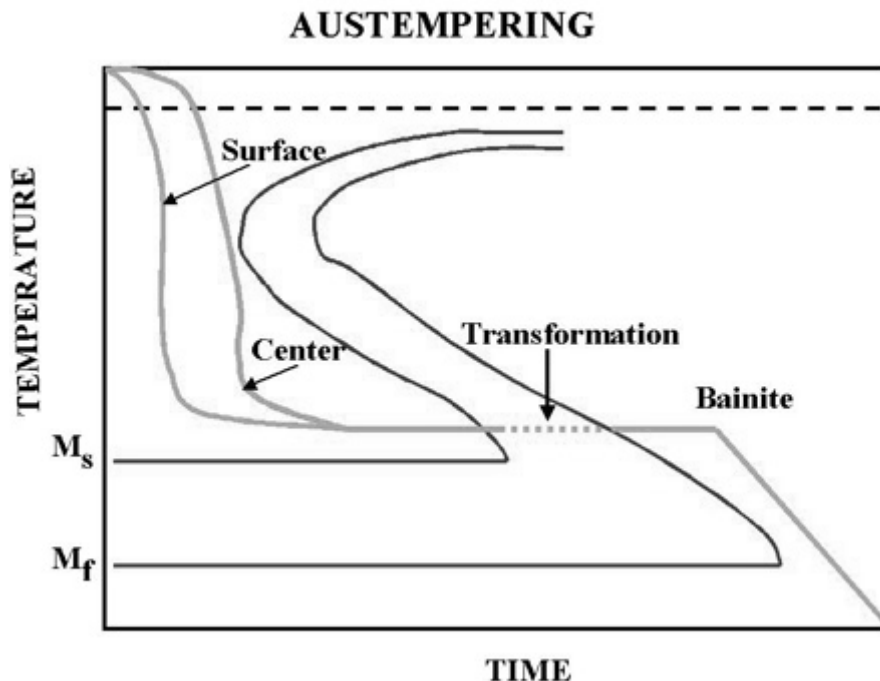
Figure 2.20 Austempering process.
