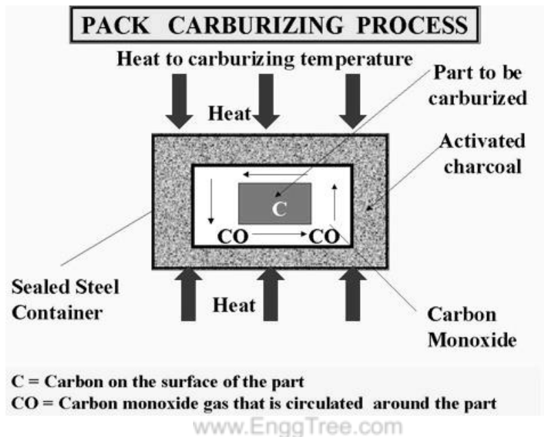
Figure 2.29 Pack carburizing process
