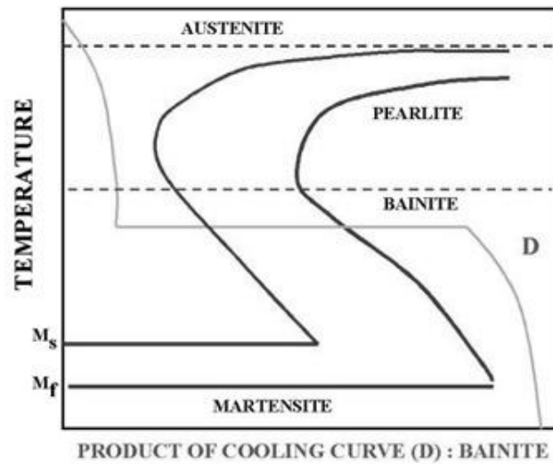
Figure 2.10 Interrupted Quench 35
