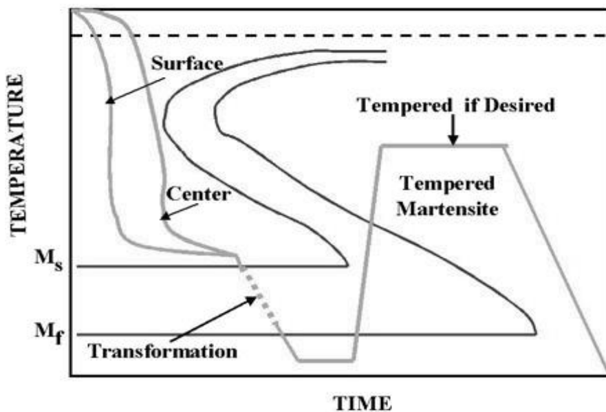
Figure 2.19 Martempering process.
