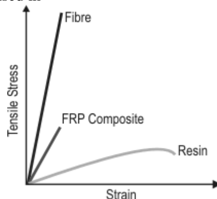
Figure 4.1 Illustrating the combined effect on Modulus of the addition of fibres to a resin matrix Overall, the properties of the composite are determined by the ,
