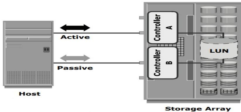
Figure 4-8: Active-passive configuration
