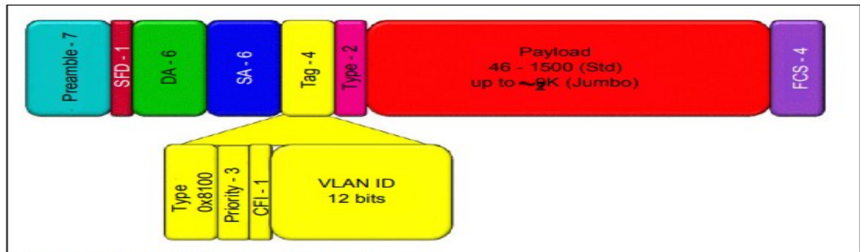
Figure 4-7 IEEE 802.1p/q tagged Ethernet frame
