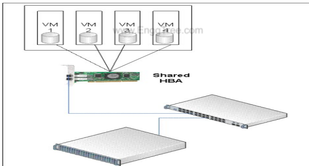
Figure 6-11 Single HBA with multiple virtual nodes
