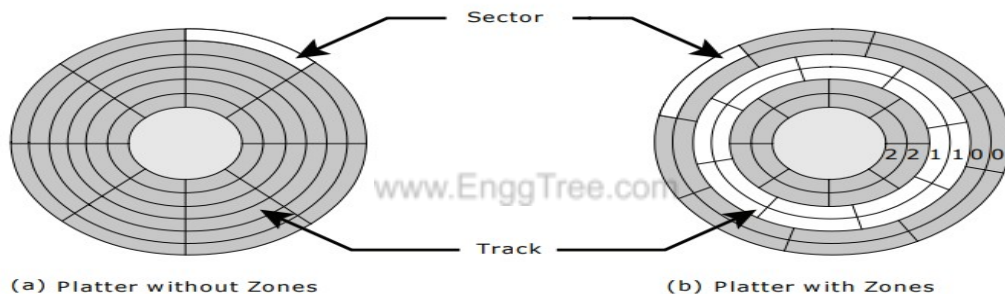
Figure 2-6: Zoned bit recording
