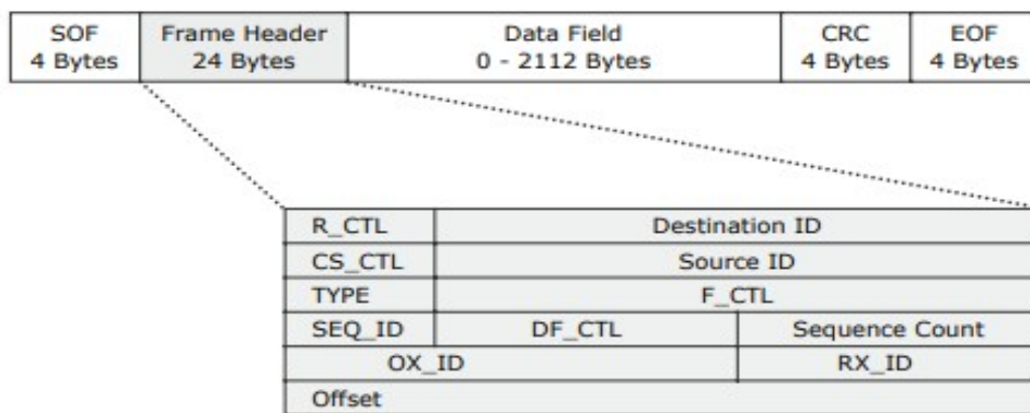
Figure 6-17: FC frame
