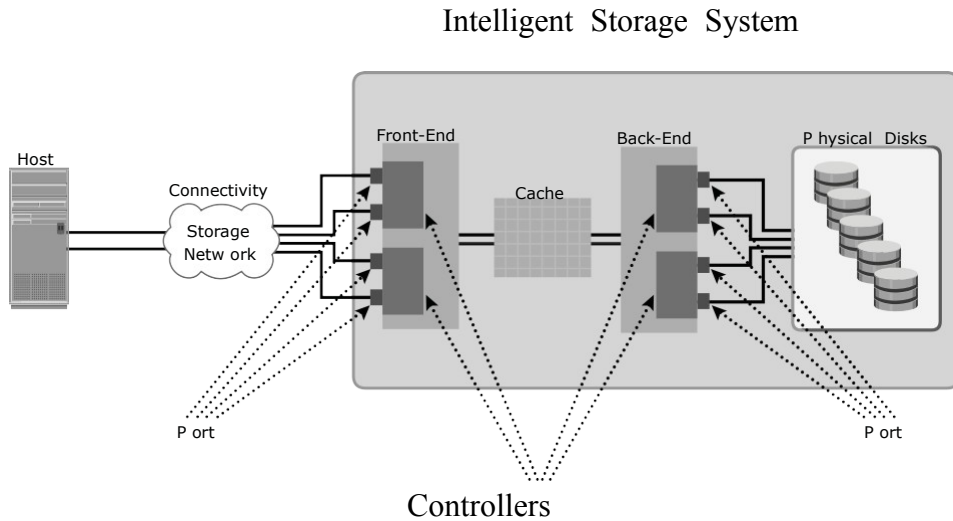
Figure 4-1: Components of an intelligent storage system
