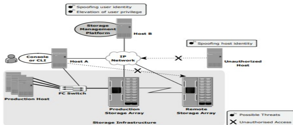
Figure 15-3: Security threats in management access domain
