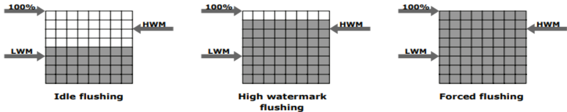
Figure 4-5: Types of flushing
