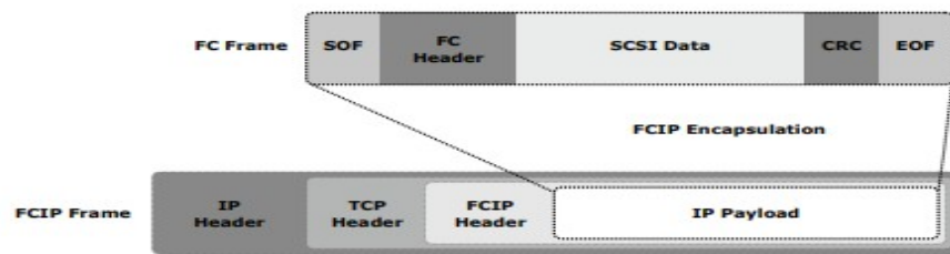
Figure 8-9: FCIP encapsulation
