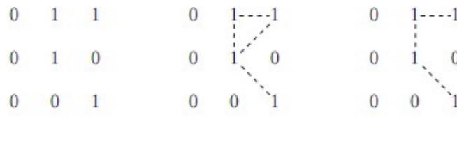
Fig.9 (a) Arrangement of pixels; (b) pixels that are 8-adjacent (shown dashed) to the center pixel; (c) m-adjacency
