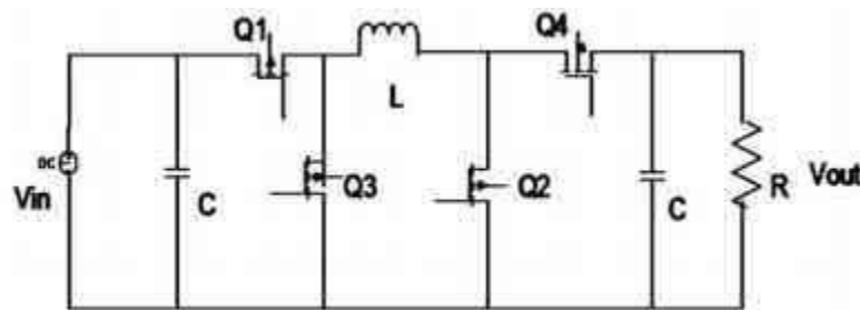
Four-switch buck-boost converter.
