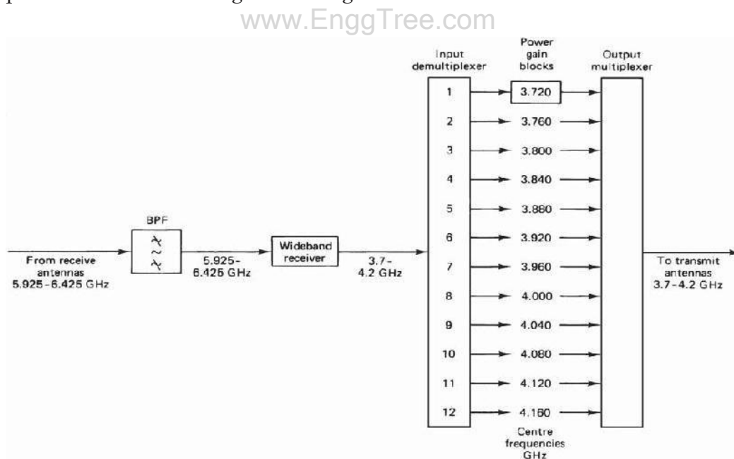
Figure 2.10 Satellite transponder channels
