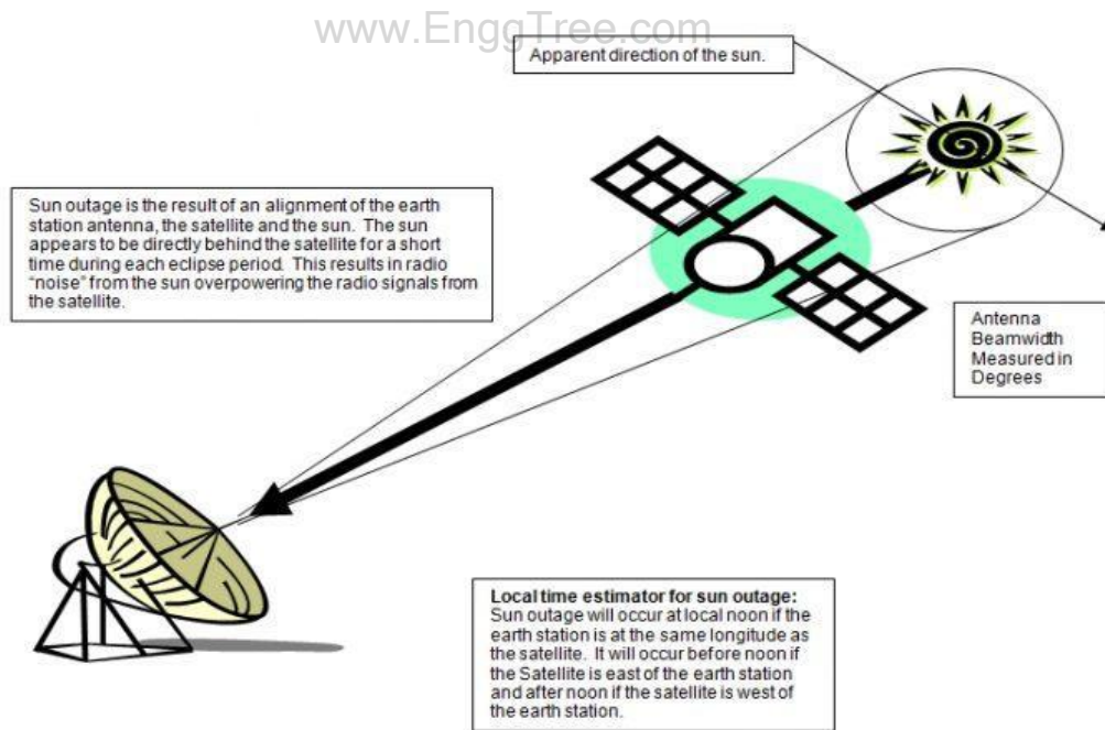
Figure example of sun transit outage
