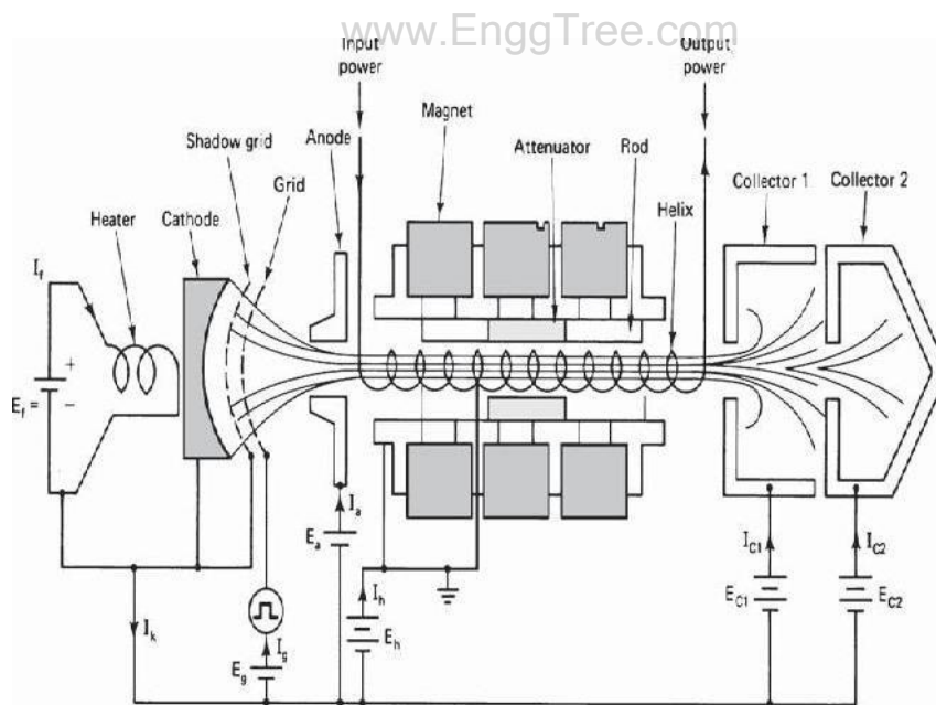
Figure 2.13 Satellite TWT
