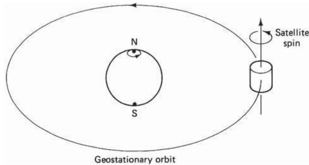
Figure 2.3 Spin stabilization in the geostationary orbit. The spin axis lies along the pitch axis, parallel to the earth's N-S axis.
