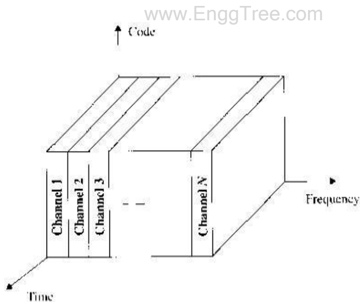
Figure 4.7 FDMA Channels
