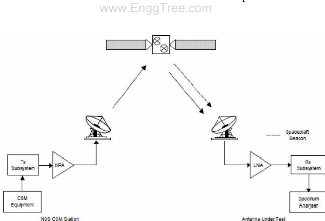
Figure 3.6 One possible arrangement for Measurement of G/T
