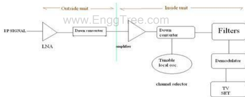
Figure 5.13 DTH Service
