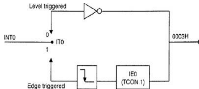
Fig. Shows the activation of INT0 and INT1
