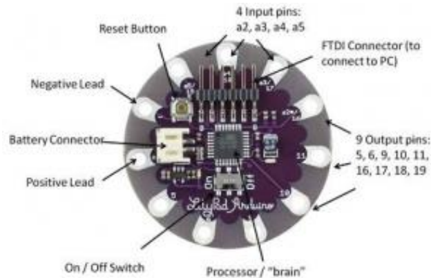
LilyPad Arduino Boards
