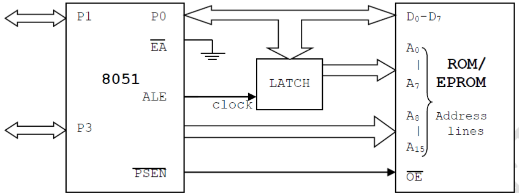
Interfacing of ROM/EPROM to 8051
