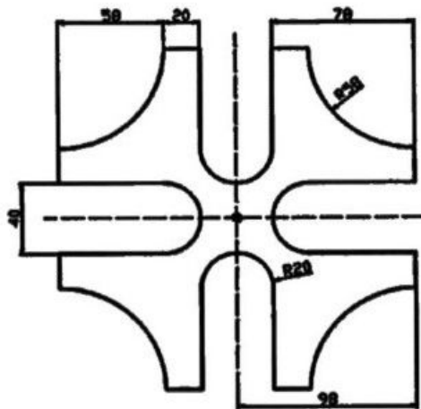
Fig. 2 : CNC program profile
